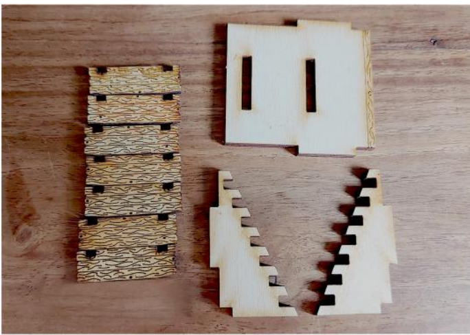
6) Layout of the parts needed to assemble the stairs for the main deck staircase. x1 Wall panel, x2 Stair wall panels, x7 Stair panels.
